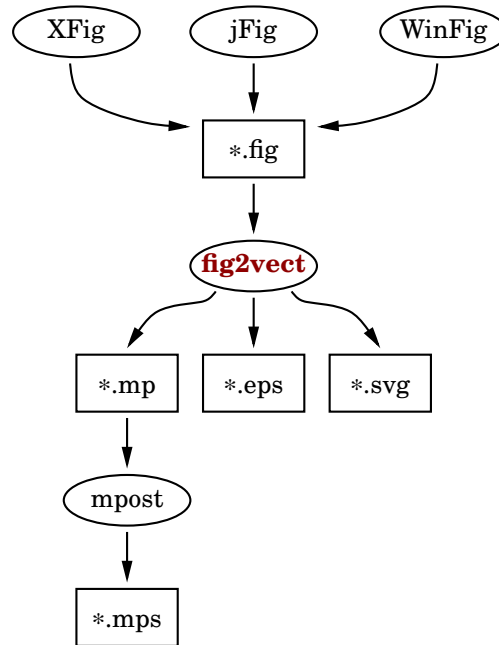
Figure 1: Data flow
