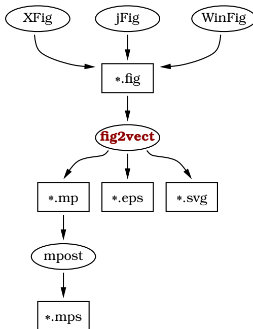
Figure 1: Data flow
